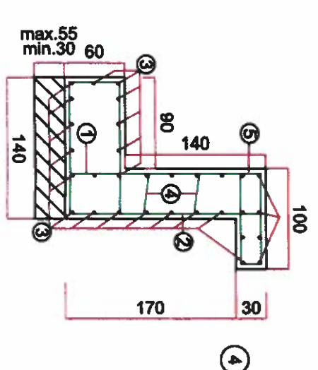
SECTION B-B SECTION 1:50
