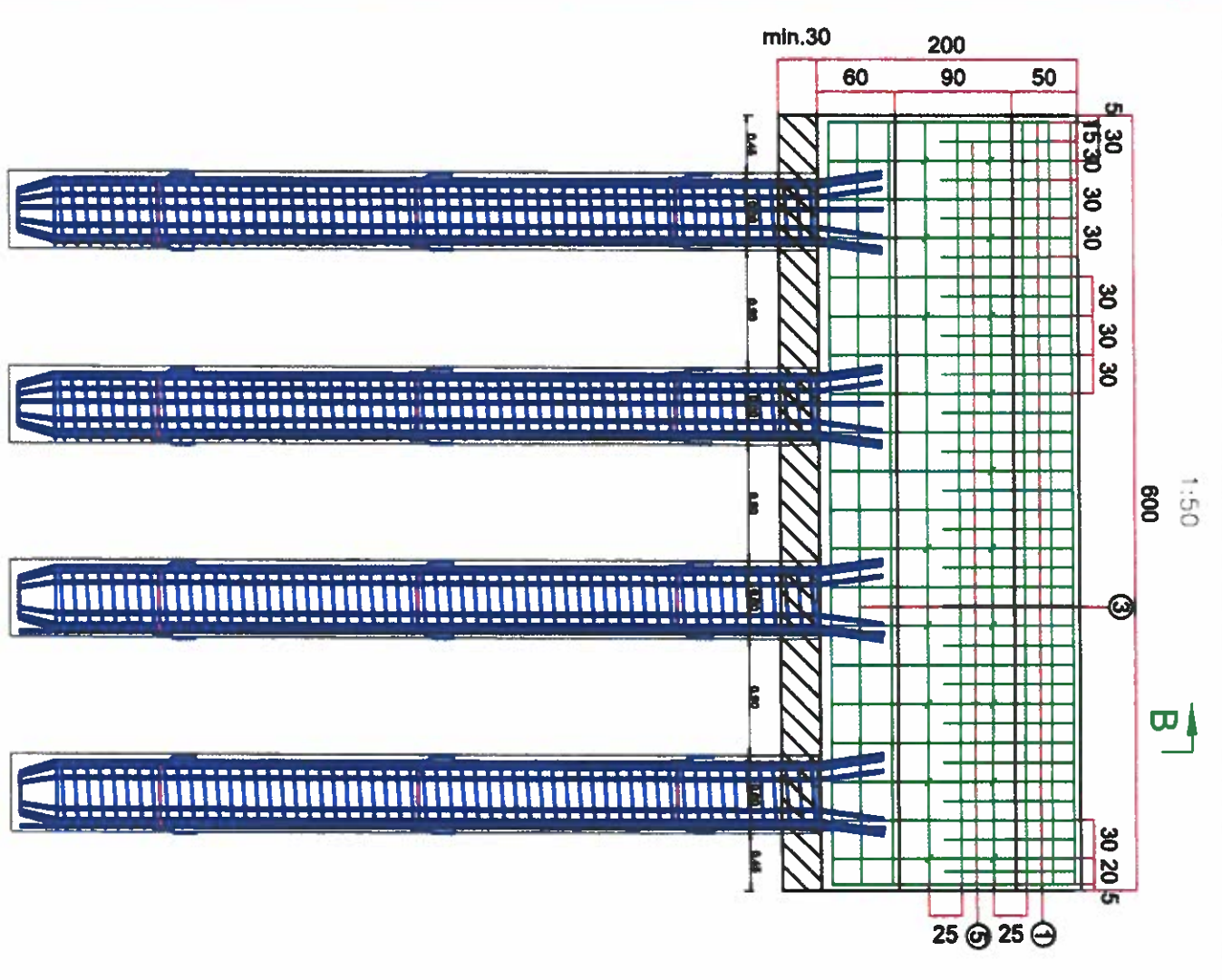
SECTION A-A SECTION 1:50
