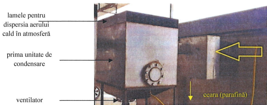
Recipient stocare parafina
