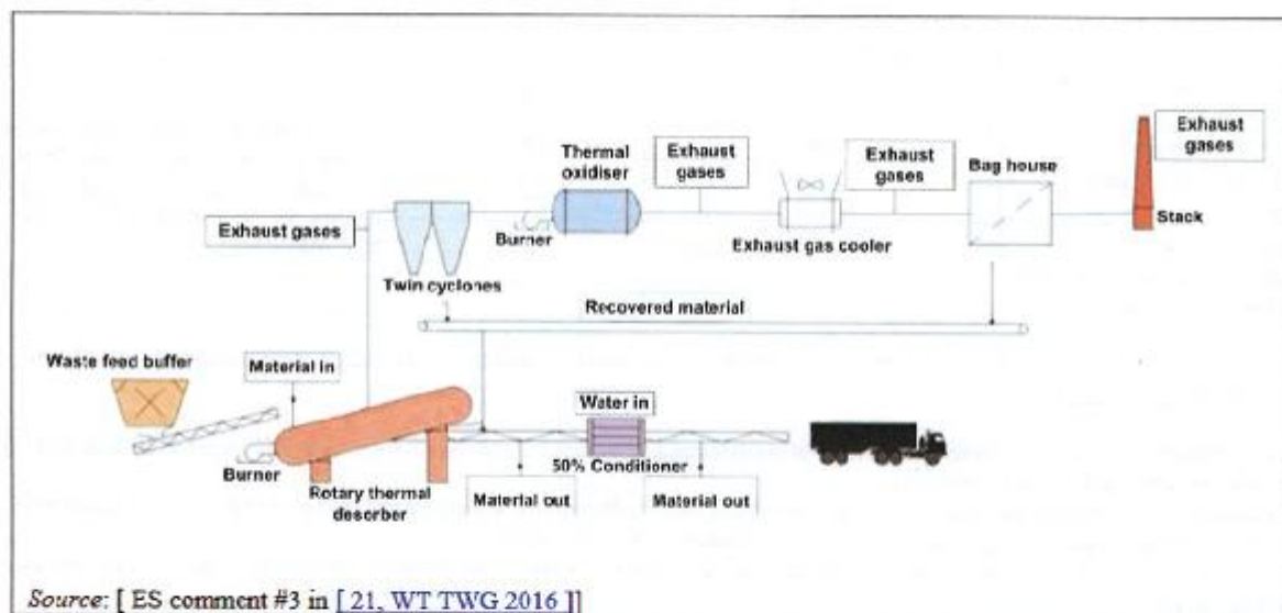
Figure 5.21: Example of a rotary thermal desorber installation
